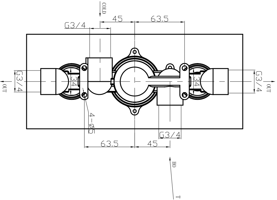
HJ2000RC - HEY JOE THERMOSTATIC SHOWER VALVE 2 Control Portrait
