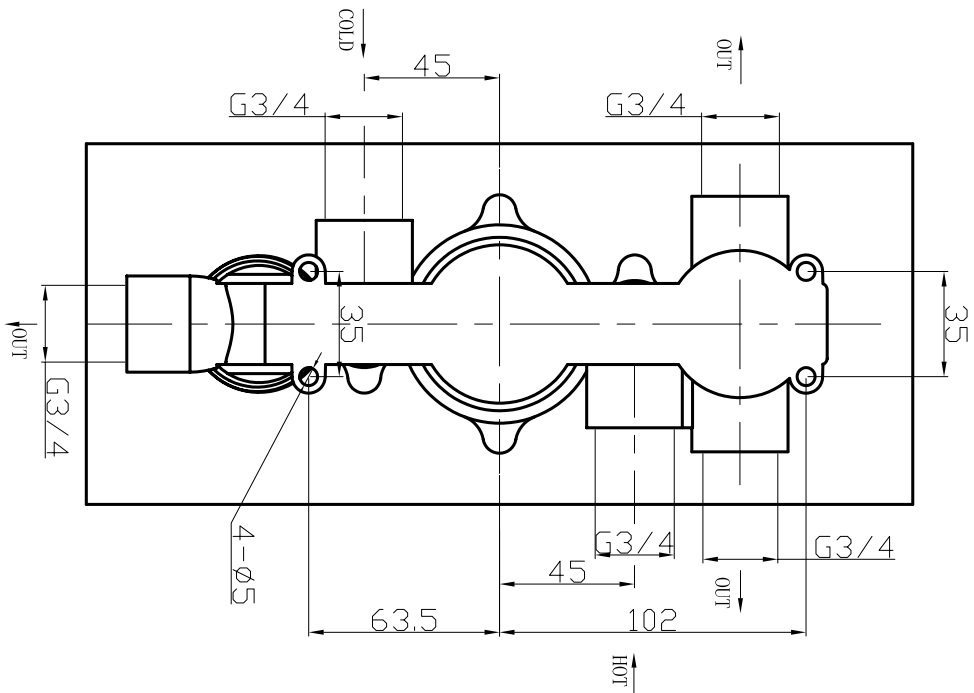
HJ3000RC - HEY JOE THERMOSTATIC SHOWER VALVE 3 Way Diverter
