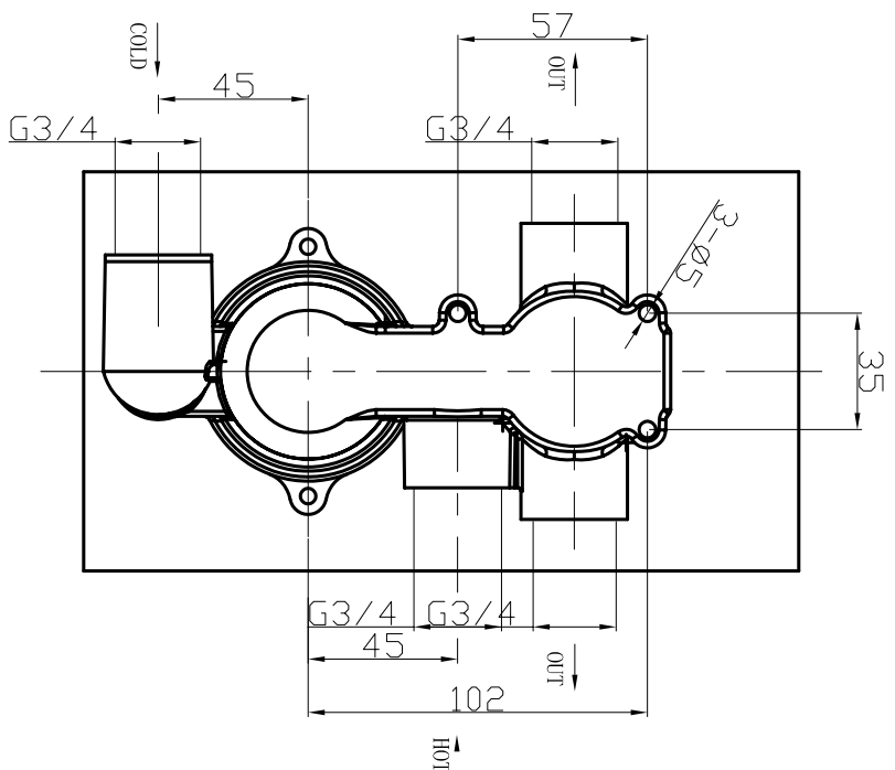
TO1500RC - TOTTI THERMOSTATIC SHOWER VALVE With 2 Way Diverter
